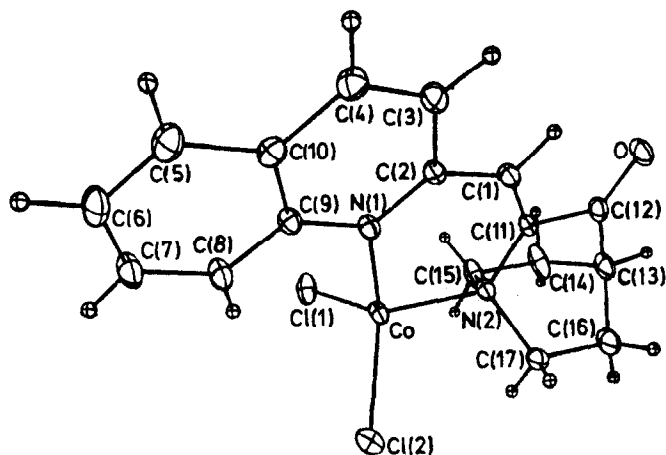
Fig. 2. The monomeric formula unit in \text{Co}(\text{qnqn})\text{Cl}_2 .
